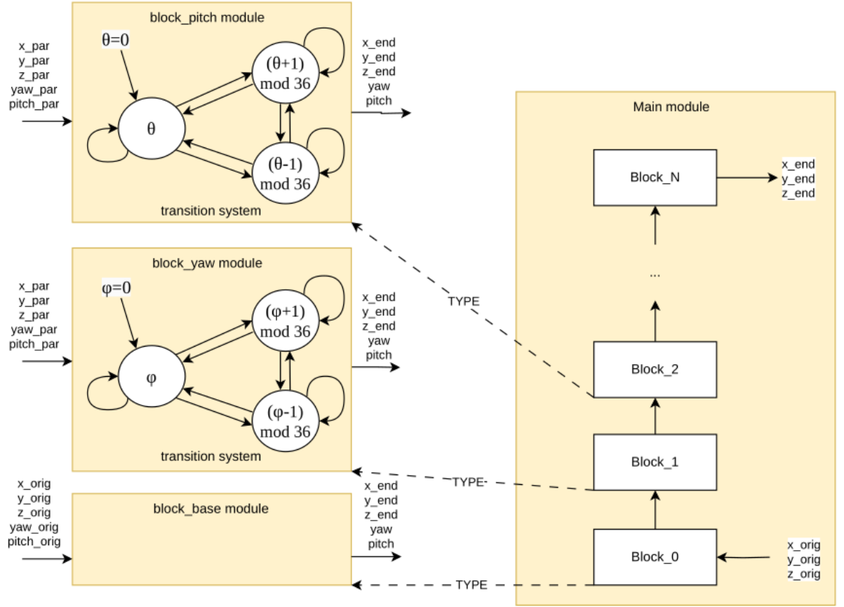
Figure 5.2: Robot configuration NuSMV model
